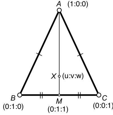
FIGURE 6. Center X of an isosceles triangle
