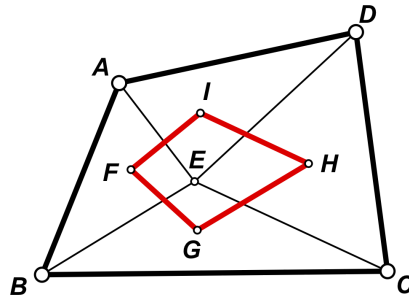
FIGURE 2. Central Quadrilateral
