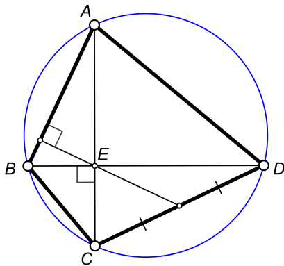
FIGURE 85. Brahmagupta's Theorem
