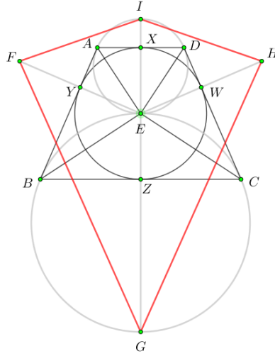
FIGURE 78. Bicentric trapezoid and incircle
