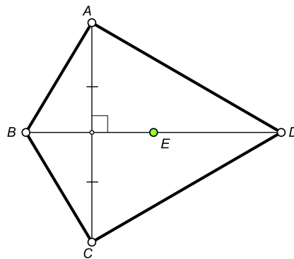
FIGURE 58. Steiner point E of kite is midpoint of BD
