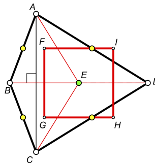
FIGURE 64. Equidiagonal kite, X_{486} points \implies [ABCD] = 2[FGHI]
