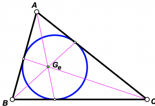
FIGURE 1. Gergonne point
