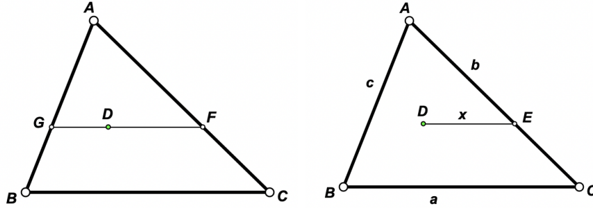
FIGURE 2. Gergonne Chord and Gergonne Pararadius
